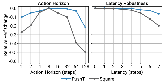
Figure 5. Diffusion Policy Ablation Study. Change (difference) in success rate relative to the maximum for each task is shown on the Y-axis. Left: trade-off between temporal consistency and responsiveness when selecting the action horizon. Right: Diffusion Policy with position control is robust against latency. Latency is defined as the number of steps between the last frame of observations to the first action that can be executed.
