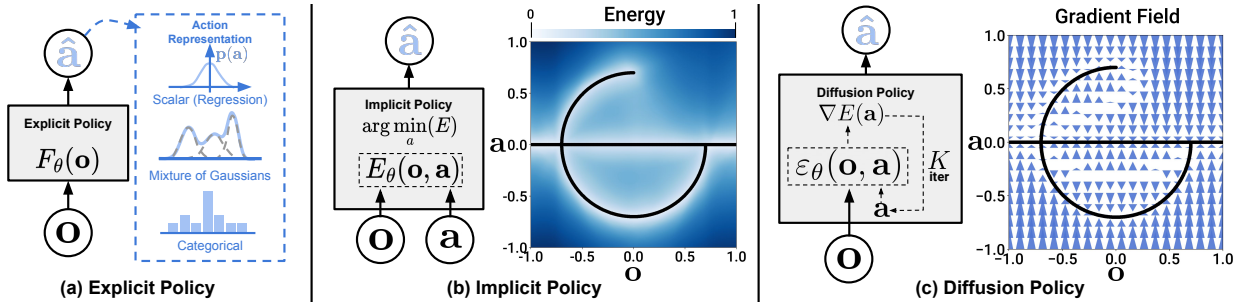
Figure 1. Diffusion Policy . a) Explicit policy with different types of action representations. b) Implicit policy learns an action score function conditioned on both action and observation and action that minimize the energy landscape c) Diffusion policy refines noise into actions via a learned gradient field. This formulation provides stable training, allows the learned policy to accurately model multimodal action distributions, and accommodates high-dimensional action sequences.
