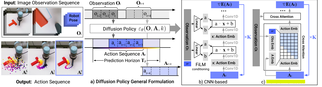
Figure 1: Diffusion Policy General Formulation and Architectures. a) General formulation. At time step t , the policy takes the latest T_o steps of observation data O_t as input and outputs T_a steps of actions A_t . b) In the CNN-based Diffusion Policy, FiLM (Feature-wise Linear Modulation) Perez et al. (2018) conditioning of the observation feature O_t is applied to every convolution layer, channel-wise. Starting from A_t^K drawn from Gaussian noise, the output of noise-prediction network \epsilon_\theta is subtracted, repeating K times to get A_t^0 , the denoised action sequence. c) In the Transformer-based Vaswani et al. (2017) Diffusion Policy, the embedding of observation O_t is passed into a [redacted] of each transformer decoder block. Each [redacted] is constrained to only attend to itself and [redacted] using the attention mask illustrated.
